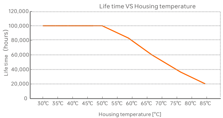
LM-150-24-G2D2F
