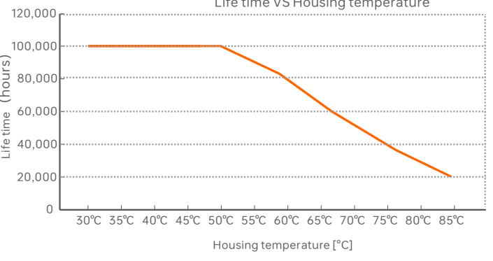
LM-150-12-G1D2F
